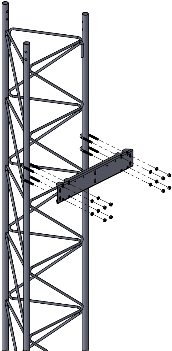
ATTACH BRACKET
